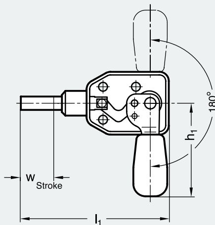
Type ASS Clamping by turning handle to the left
