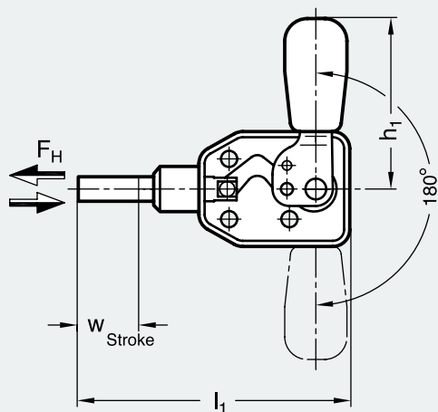
Type ASD Clamping by turning handle to the right
