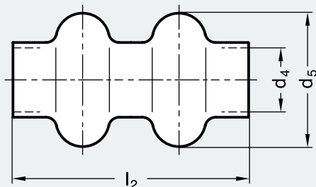
Type E for single joints
